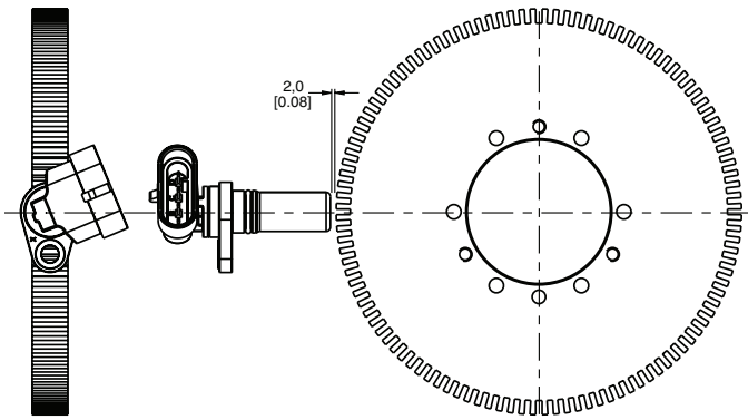
Figure 6. SNG-QPRA-000 Mounting Dimensions (For reference only: mm/[in].)
